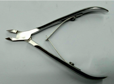
Article No 27-147 nail nipper 10.5 cm/ Tip 5mm, lap joint double spring steel grade AISI J 420 / Satin finish, Hardness 49 to 51 HRC
